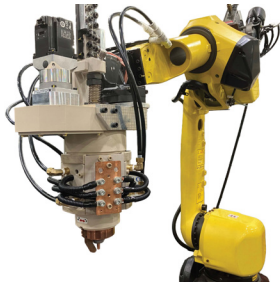
Enabling defect-free welding and printing with RotoTIG, powered by proprietary technology and the world's first center-wire-fed TIG welding torch
